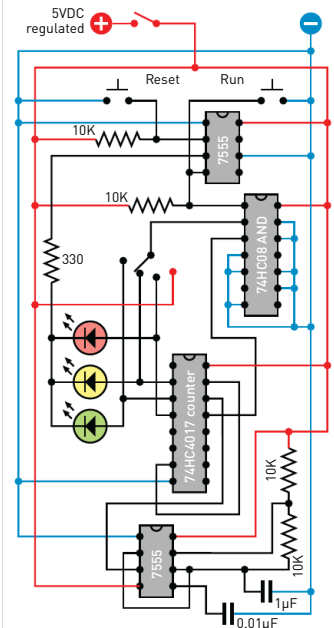
B Schematic layout suitable for breadboarding.
