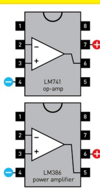
Basic pinouts of the LM741 op-amp and LM386 power amp. Unlabeled pins have additional functions; see datasheets for details.
