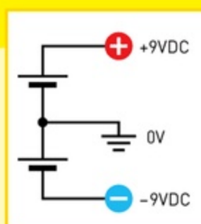
D The split power supply required by the circuit can be provided by two 9V batteries wired in series.
