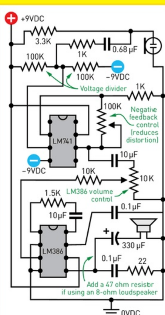
C An audio amplifier circuit.
