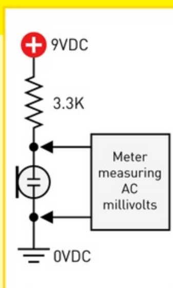
B Detecting the output from an electret microphone.
