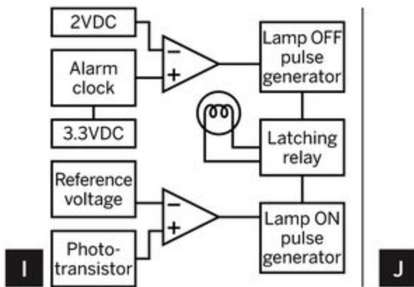
The main circuit, omitting the power supply in Figure E.
