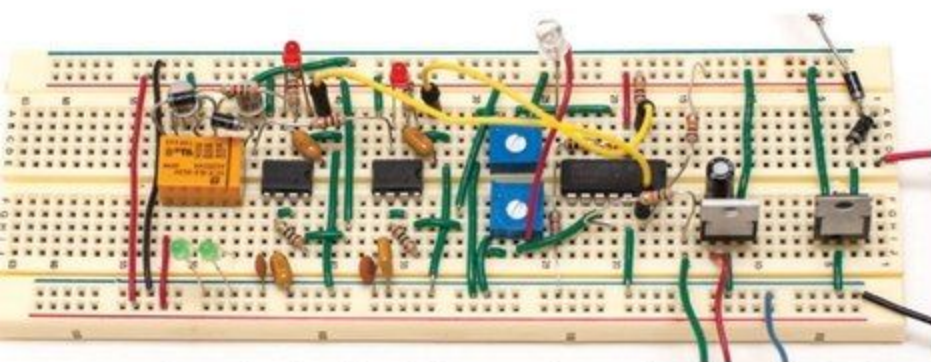
A complete breadboarded circuit showing the orange relay with input transistors and 2 green test LEDs, two 555 timers with red test LEDs, blue trimmer potentiometers, LM339 quad comparator chip, and voltage regulators for 3.3VDC and 5VDC.
