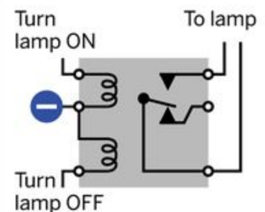
K Relay viewed from above
